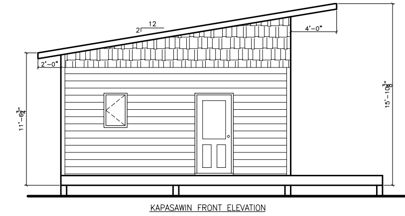
KAPASAWIN FRONT ELEVATION
